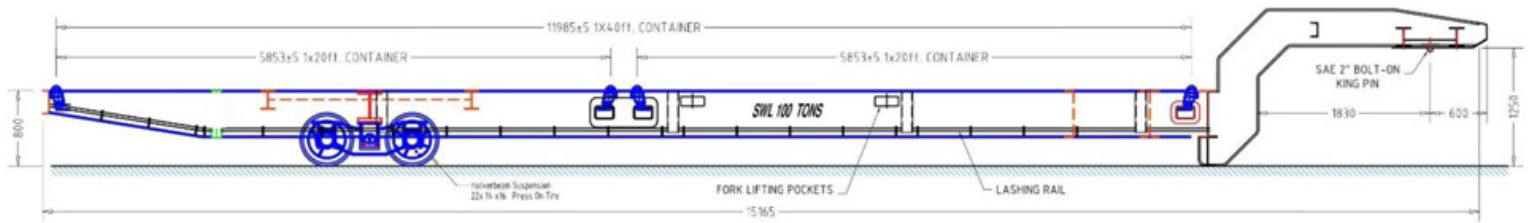
SIDE VIEW
