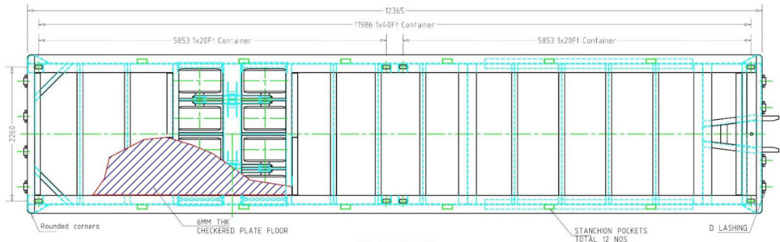
PLAN VIEW
